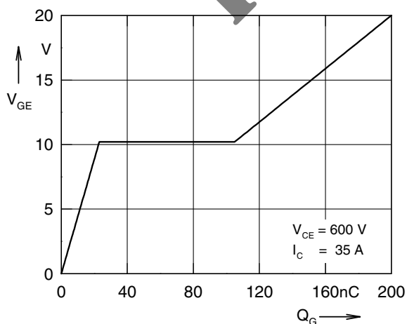
Fig. 11 Typ. turn on gate charge
